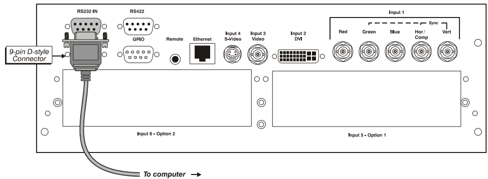
Figure 2.10. Connecting RS232
